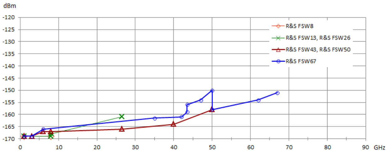
Typical displayed average noise level of the FSW models for f > 1 GHz with R&S®FSW-B24 12 RF preamplifier option, preamplifier gain = 30 dB
