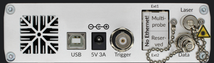
Computer Interface Rear Side View
